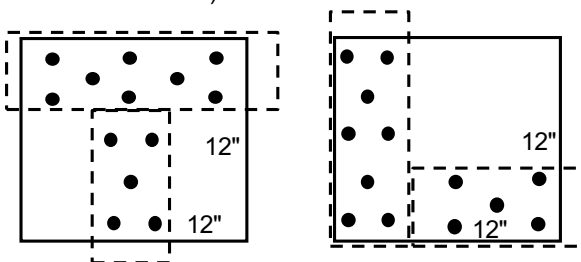
T-Shore – Header/Post
