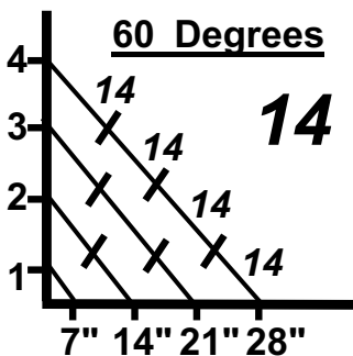
RAKER LENGTH BASED ON INSERTION POINT HEIGHT
